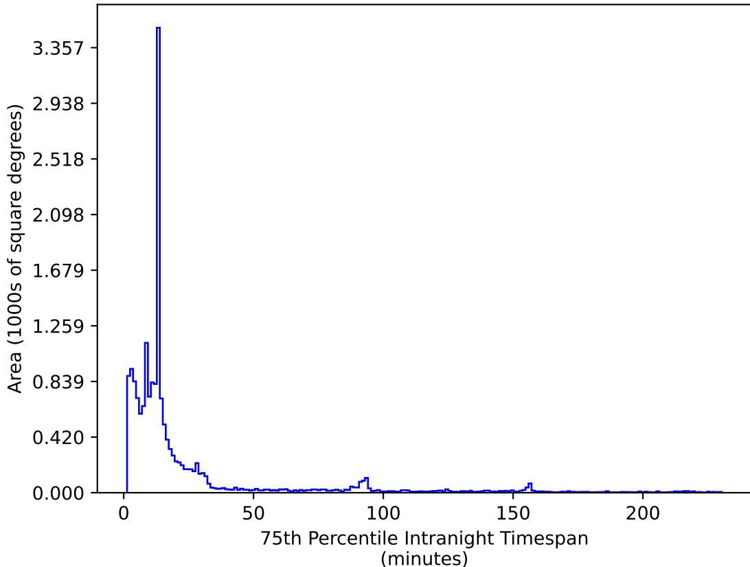
roll_pause_mjdp0_v3.4_10yrs WFD i band: 75th Percentile Intranight Timespan
