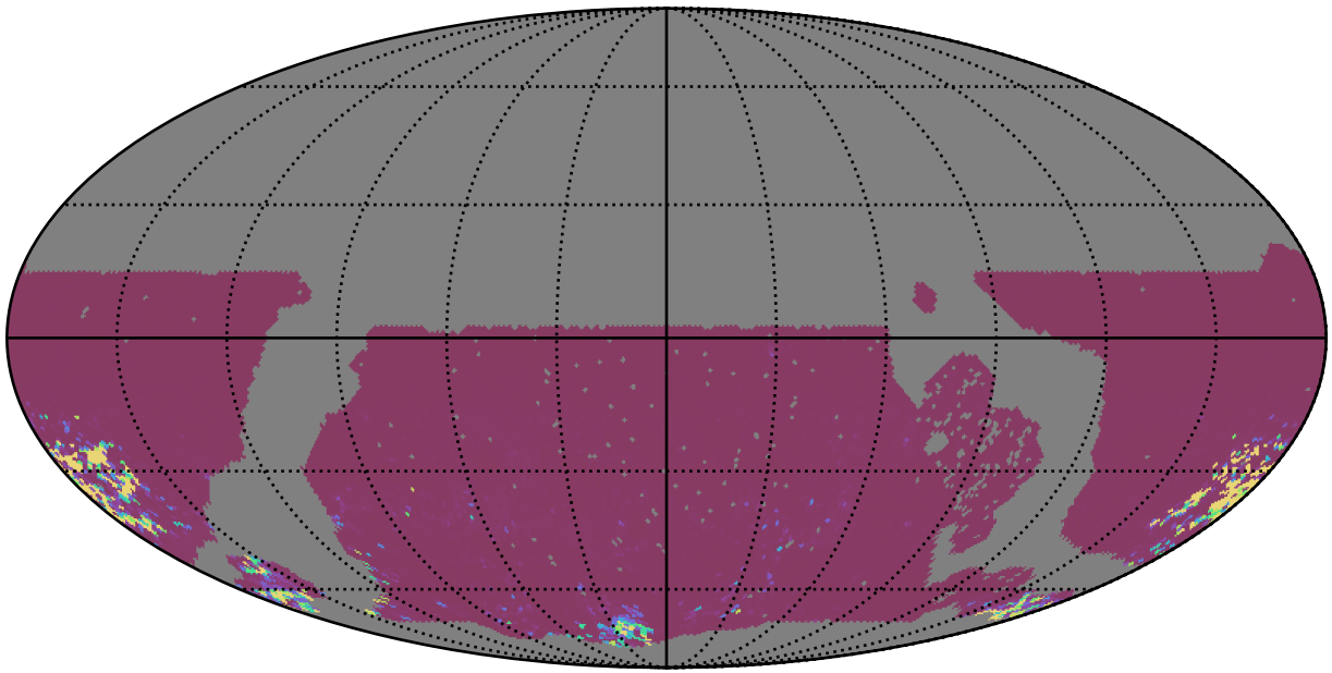
roll_pause_mjdp0_v3.4_10yrs WFD gr bands: 75th Percentile Intranight Timespan
