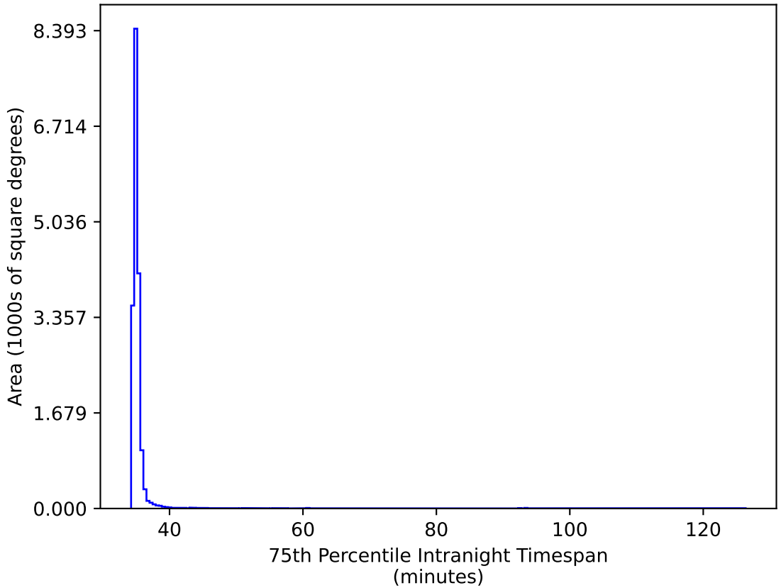
roll_pause_mjdp0_v3.4_10yrs WFD gr bands: 75th Percentile Intranight Timespan
