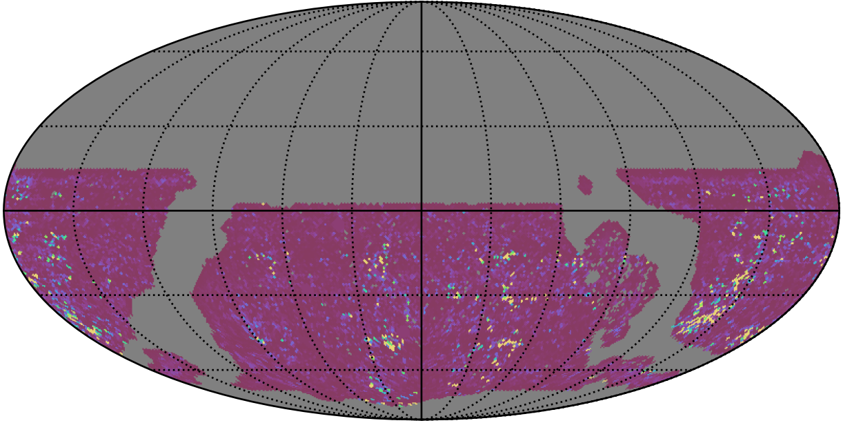
roll_pause_mjdp0_v3.4_10yrs WFD g band: 75th Percentile Intranight Timespan
