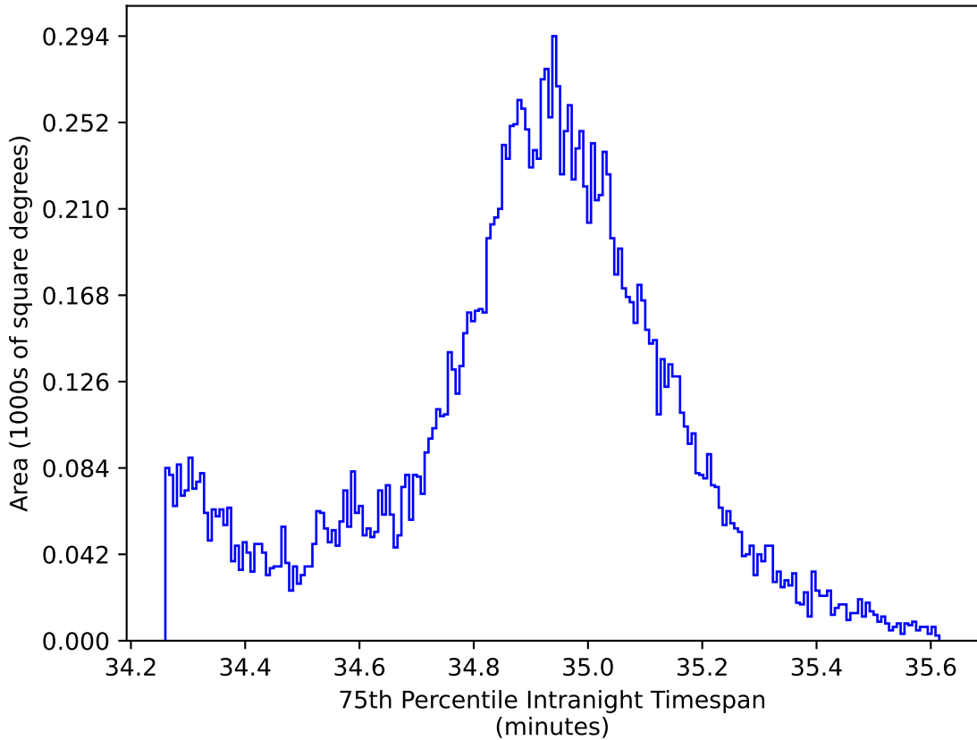
roll_pause_mjdp0_v3.4_10yrs WFD: 75th Percentile Intranight Timespan
