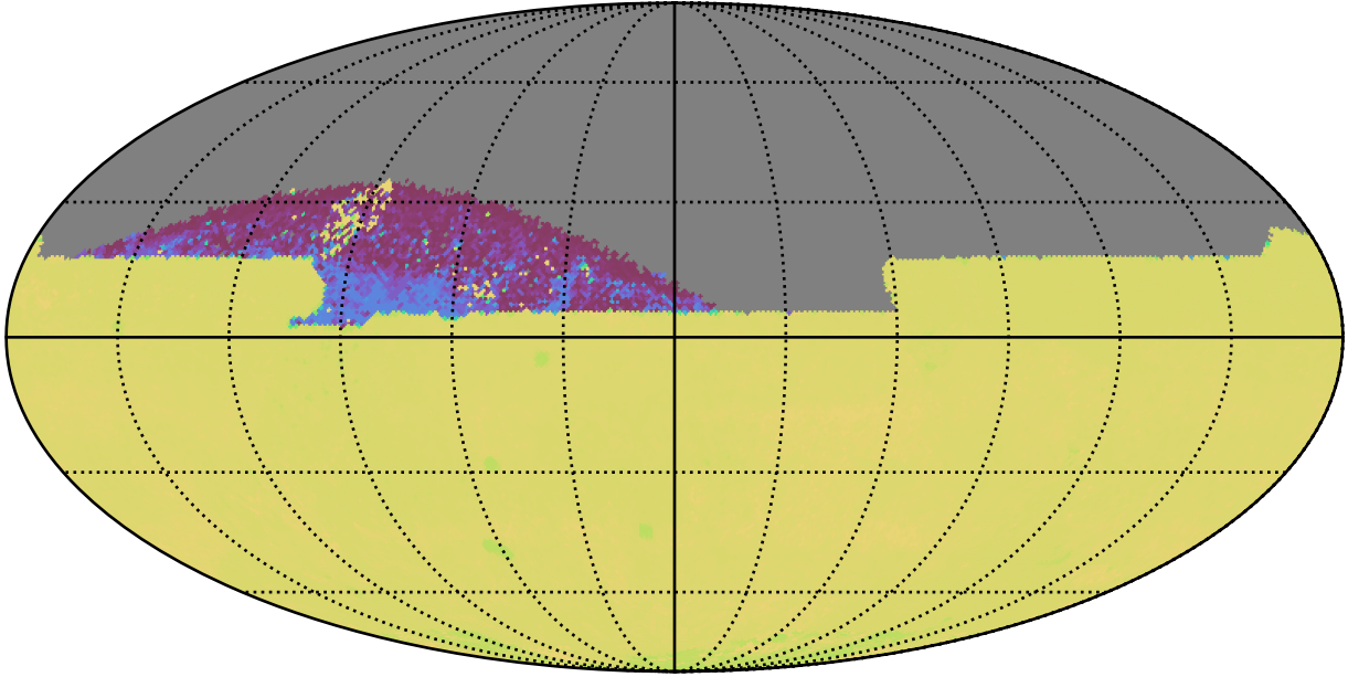
roll_pause_mjdp0_v3.4_10yrs All sky zy bands: 75th Percentile Intranight Timespan
