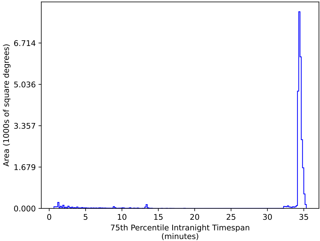
roll_pause_mjdp0_v3.4_10yrs All sky zy bands: 75th Percentile Intranight Timespan
