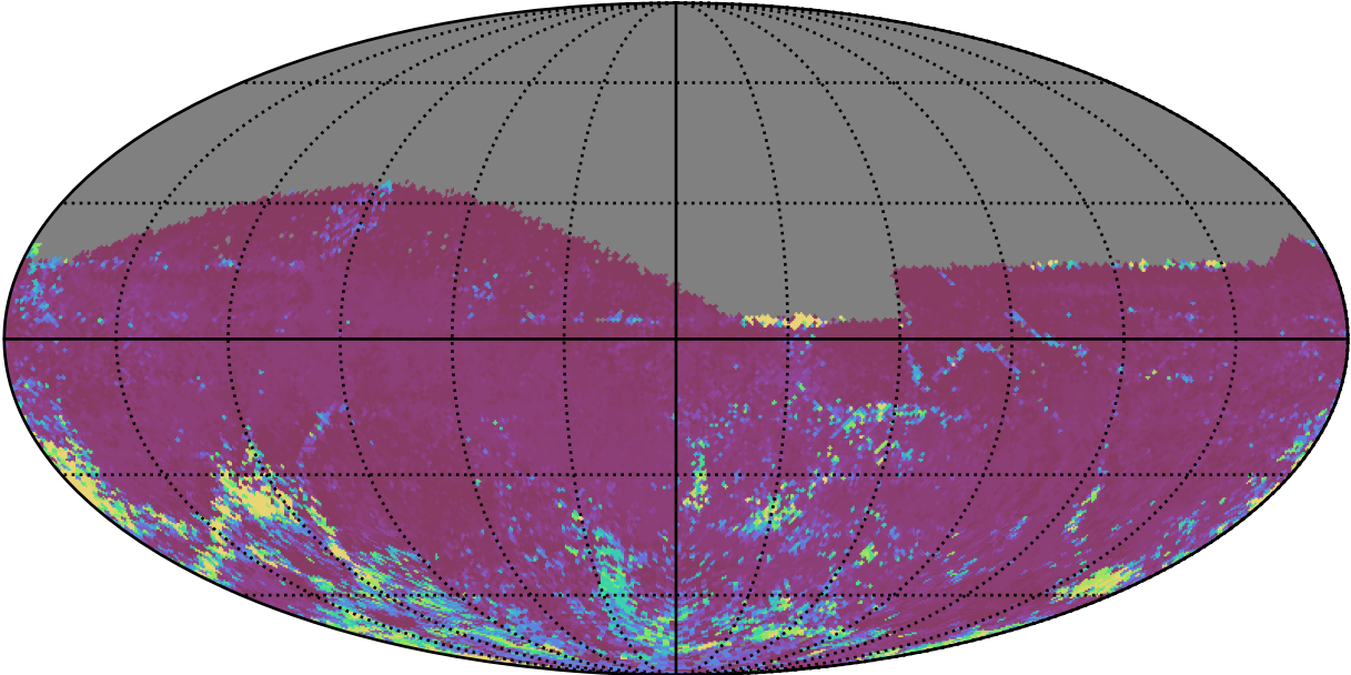
roll_pause_mjdp0_v3.4_10yrs All sky z band: 75th Percentile Intranight Timespan
