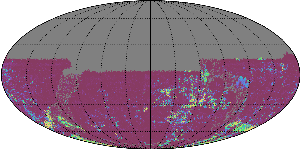
roll_pause_mjdp0_v3.4_10yrs All sky u band: 75th Percentile Intranight Timespan
