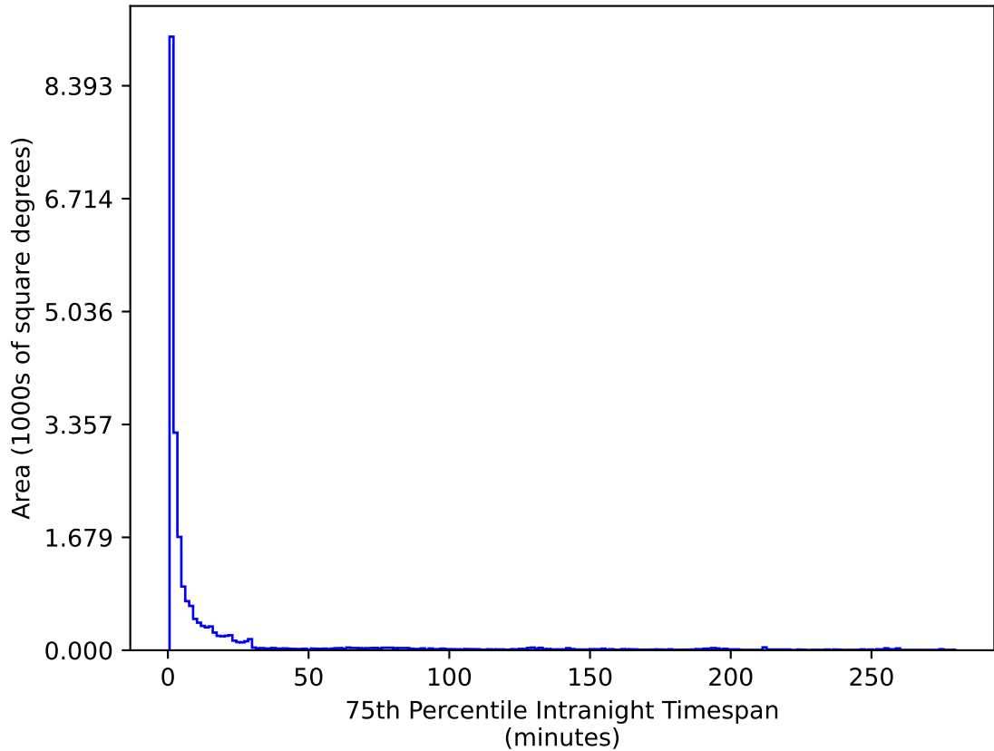
roll_pause_mjdp0_v3.4_10yrs All sky u band: 75th Percentile Intranight Timespan
