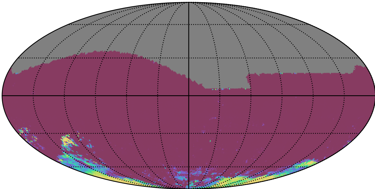
roll_pause_mjdp0_v3.4_10yrs All sky ri bands: 75th Percentile Intranight Timespan
