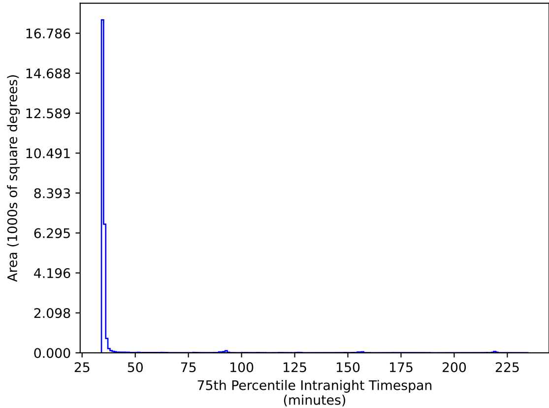
roll_pause_mjdp0_v3.4_10yrs All sky ri bands: 75th Percentile Intranight Timespan
