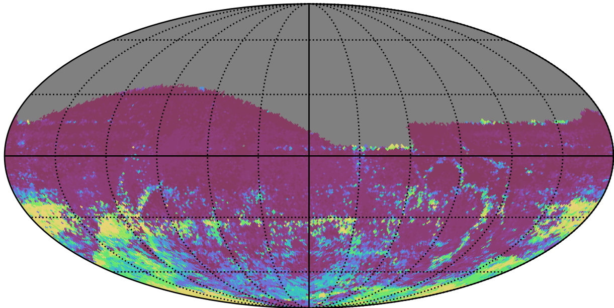
roll_pause_mjdp0_v3.4_10yrs All sky r band: 75th Percentile Intranight Timespan
