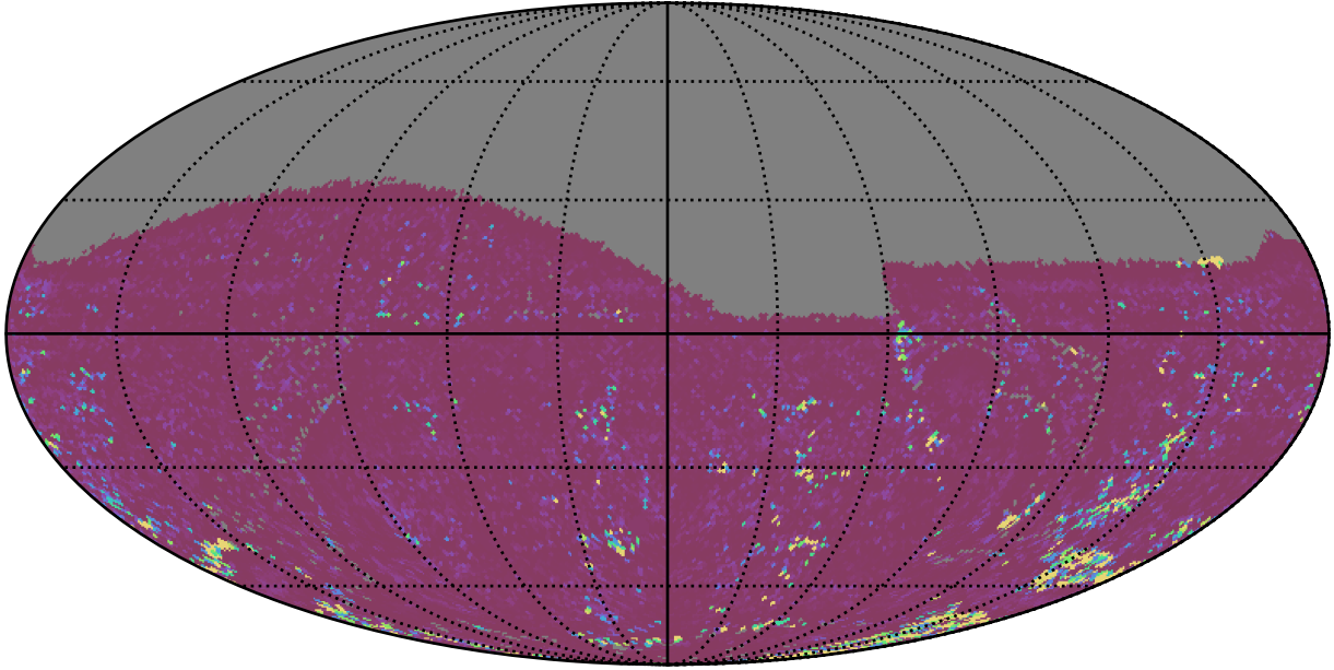
roll_pause_mjdp0_v3.4_10yrs All sky g band: 75th Percentile Intranight Timespan
