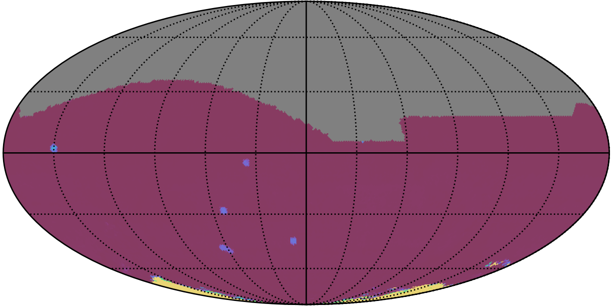
roll_pause_mjdp0_v3.4_10yrs All sky all bands: 75th Percentile Intranight Timespan
