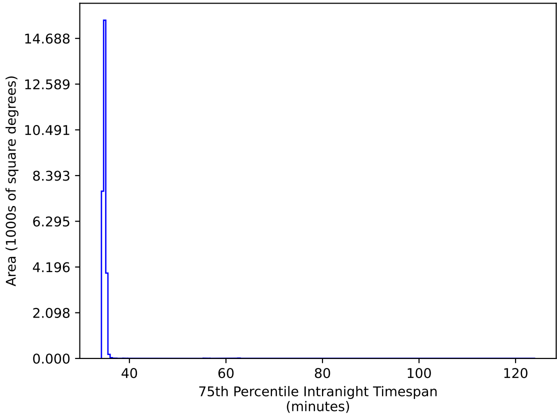
roll_pause_mjdp0_v3.4_10yrs All sky all bands: 75th Percentile Intranight Timespan
