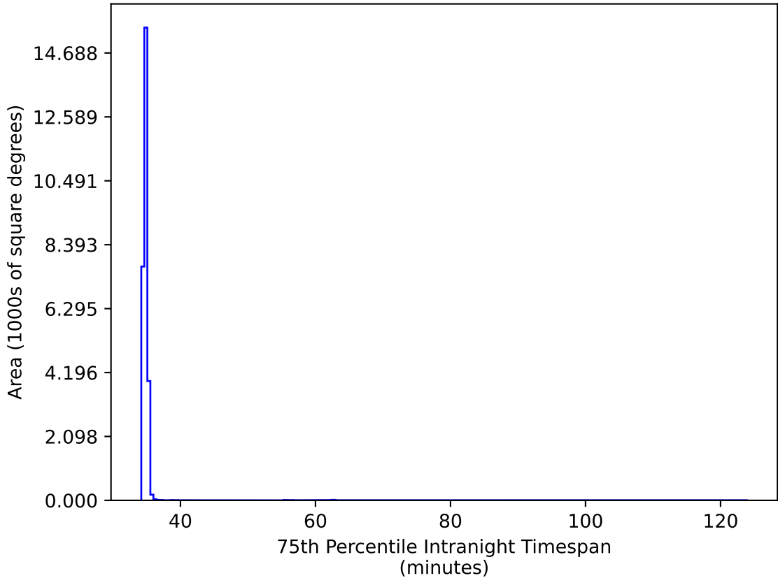
roll_pause_mjdp0_v3.4_10yrs All sky: 75th Percentile Intranight Timespan
