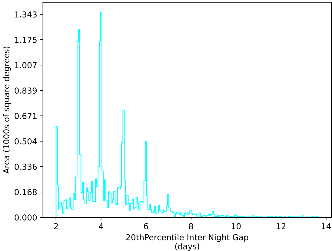
roll_pause_mjdp0_v3.4_10yrs WFD u band: 20thPercentile Inter-Night Gap
