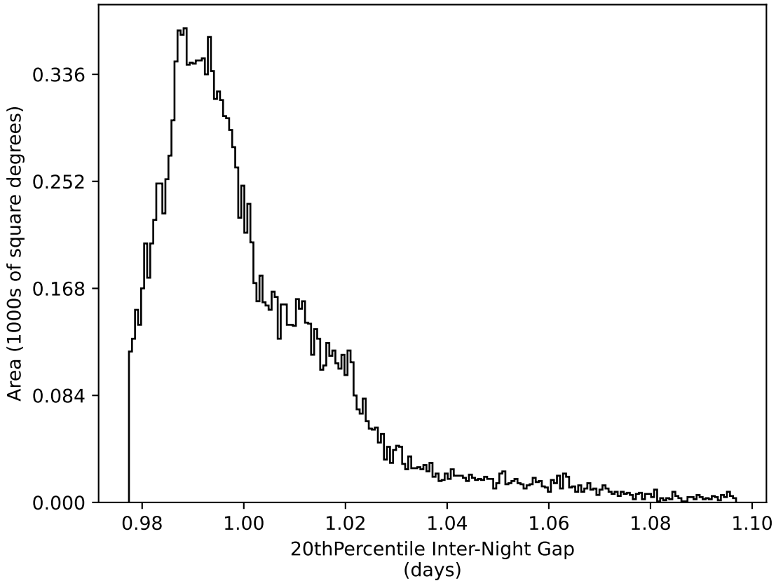
roll_pause_mjdp0_v3.4_10yrs WFD all bands: 20thPercentile Inter-Night Gap
