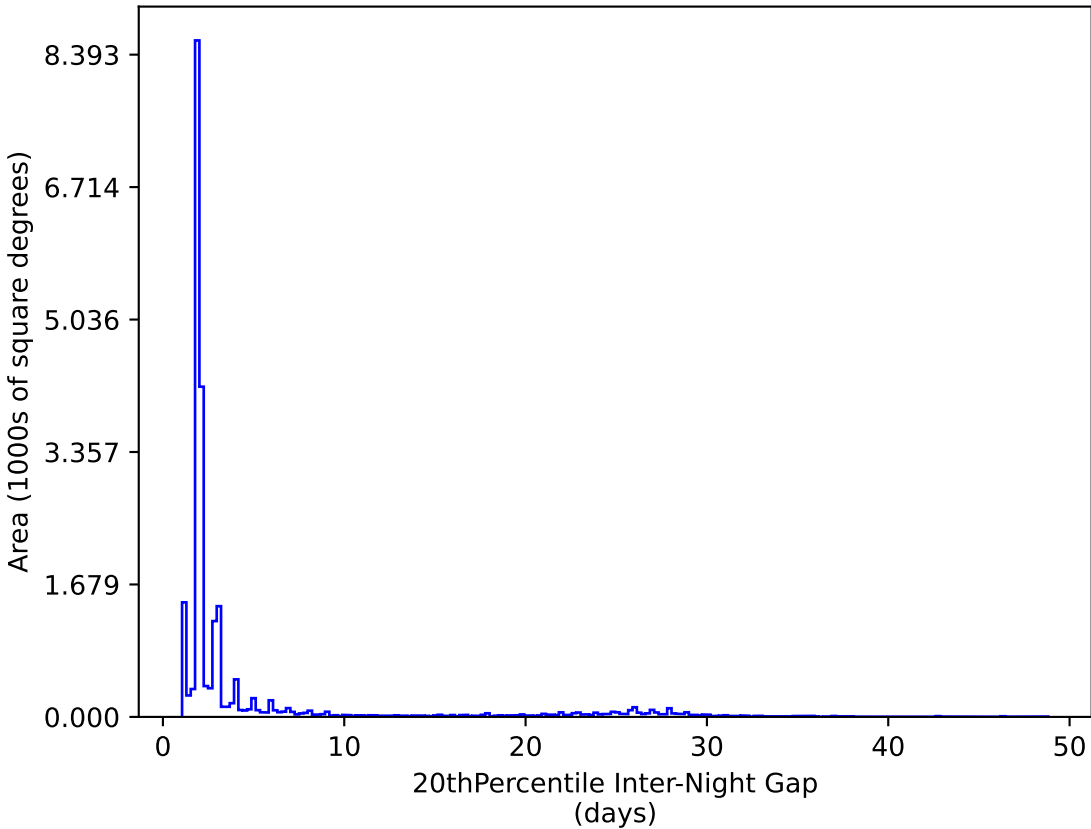
roll_pause_mjdp0_v3.4_10yrs All sky y band: 20thPercentile Inter-Night Gap
