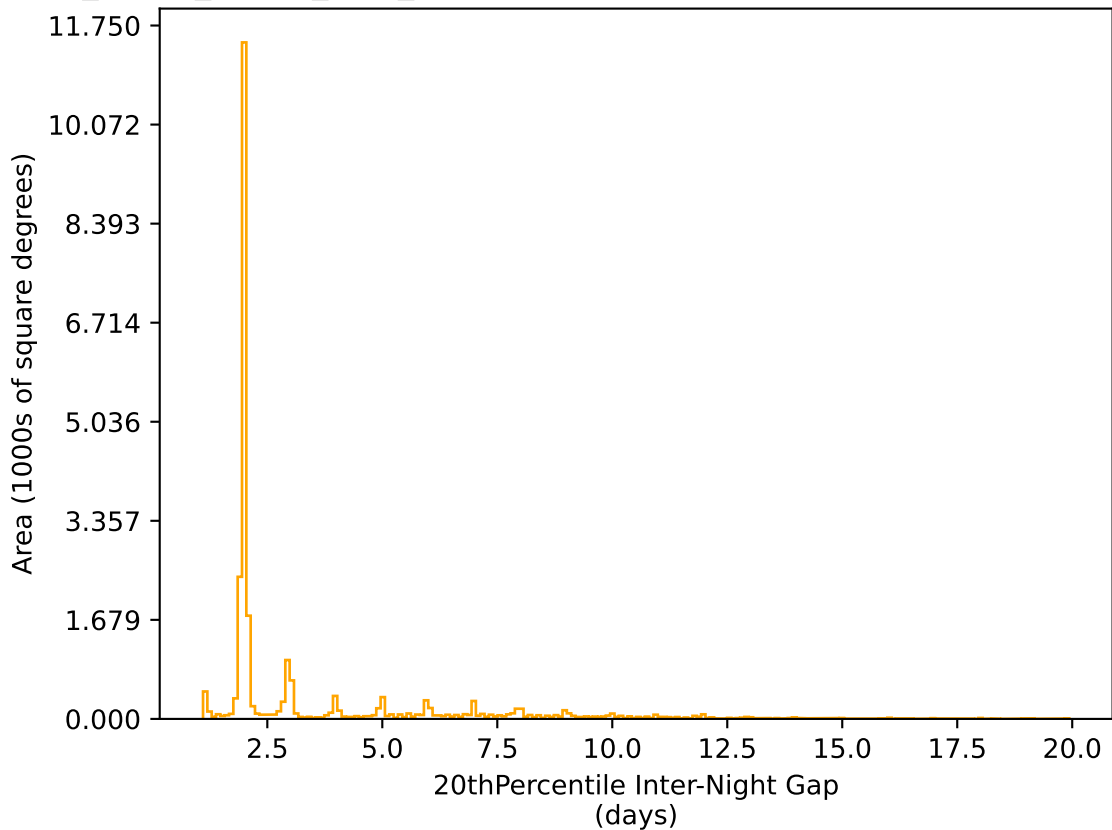
roll_pause_mjdp0_v3.4_10yrs All sky r band: 20thPercentile Inter-Night Gap
