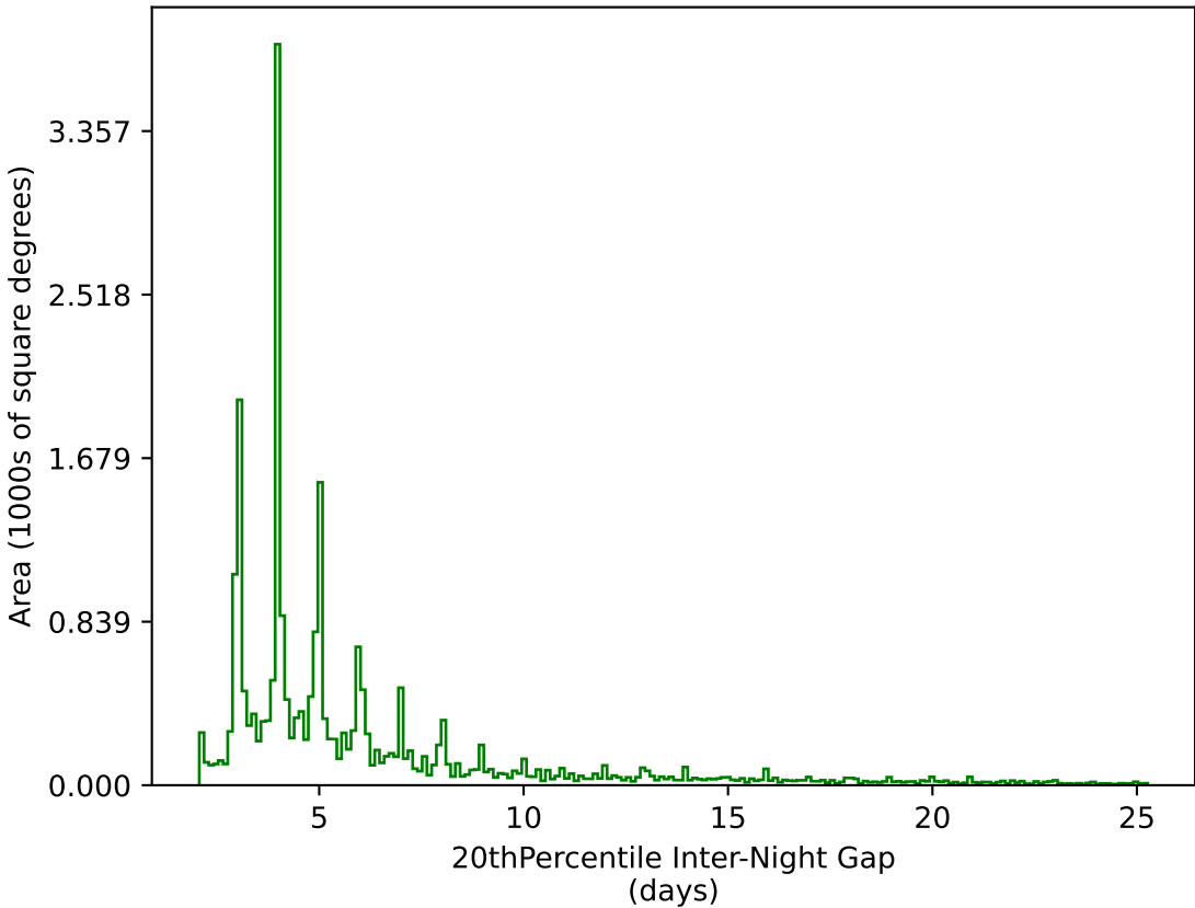
roll_pause_mjdp0_v3.4_10yrs All sky g band: 20thPercentile Inter-Night Gap
