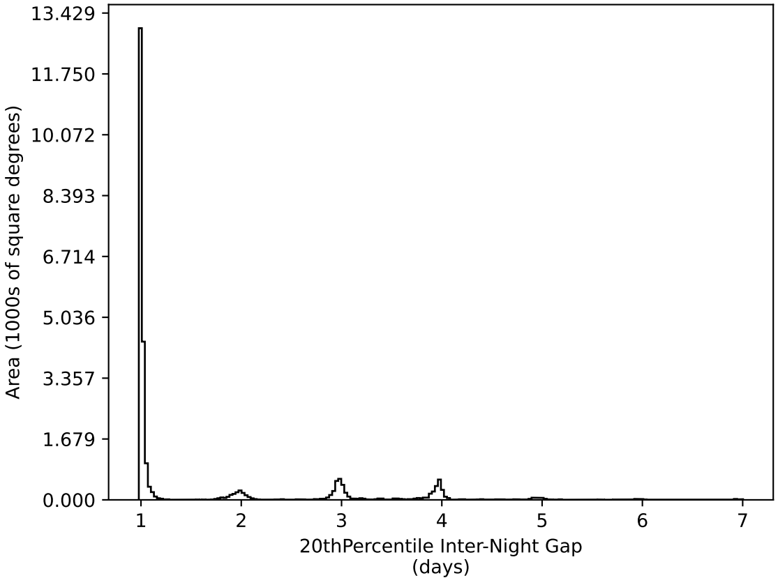
roll_pause_mjdp0_v3.4_10yrs All sky all bands: 20thPercentile Inter-Night Gap
