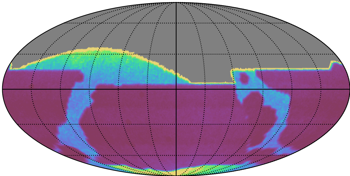
roll_pause_mjdp0_v3.4_10yrs : properMotion
