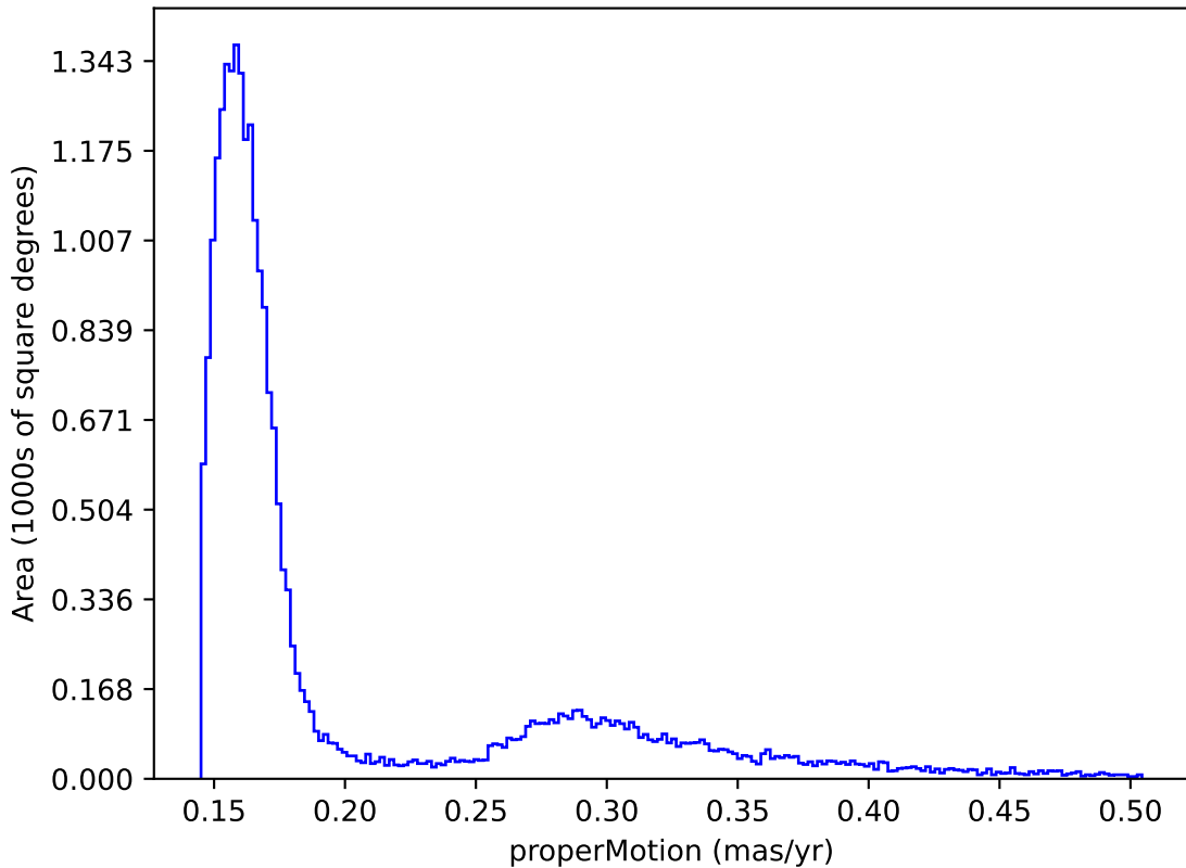
roll_pause_mjdp0_v3.4_10yrs : properMotion
