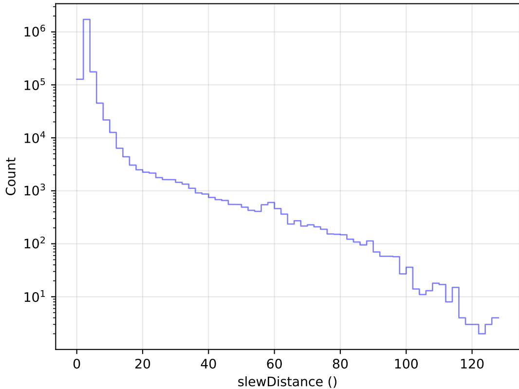
roll_pause_mjdp0_v3.4_10yrs All visits: Slew Distance Histogram
