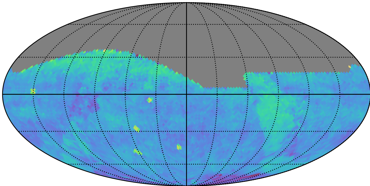
roll_pause_mjdp0_v3.4_10yrs (g or r or i): PairFraction
