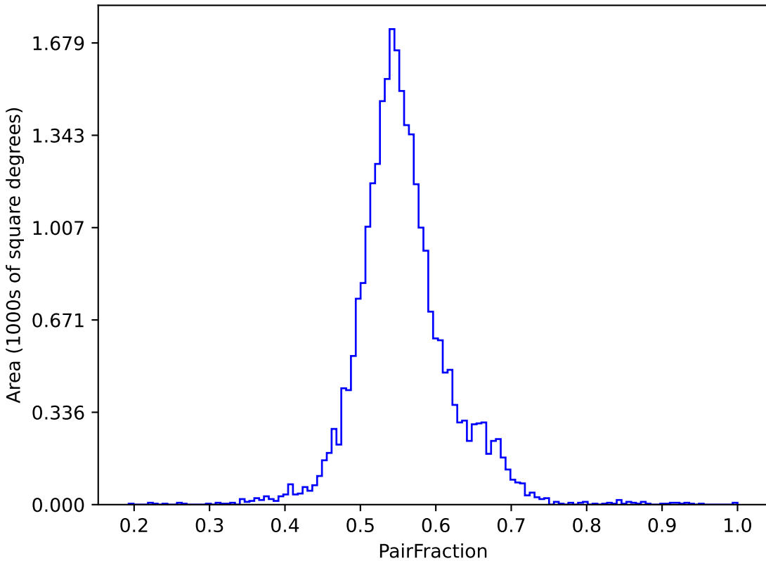
roll_pause_mjdp0_v3.4_10yrs (g or r or i): PairFraction
