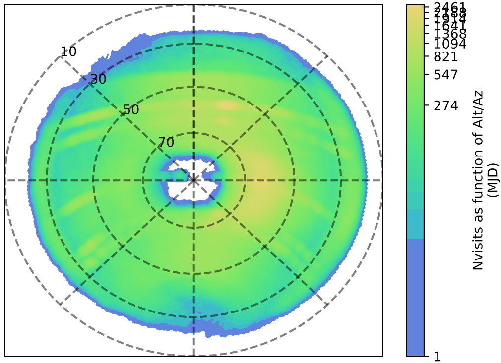
roll_pause_mjdp0_v3.4_10yrs z: Nvisits as function of Alt/Az
