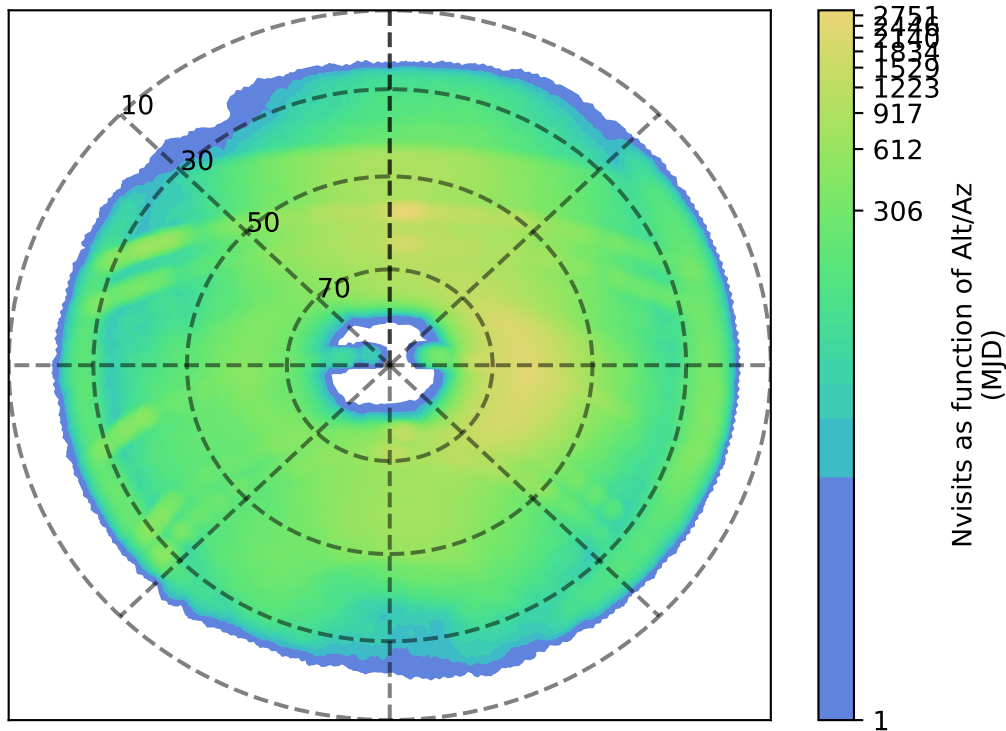
roll_pause_mjdp0_v3.4_10yrs i: Nvisits as function of Alt/Az
