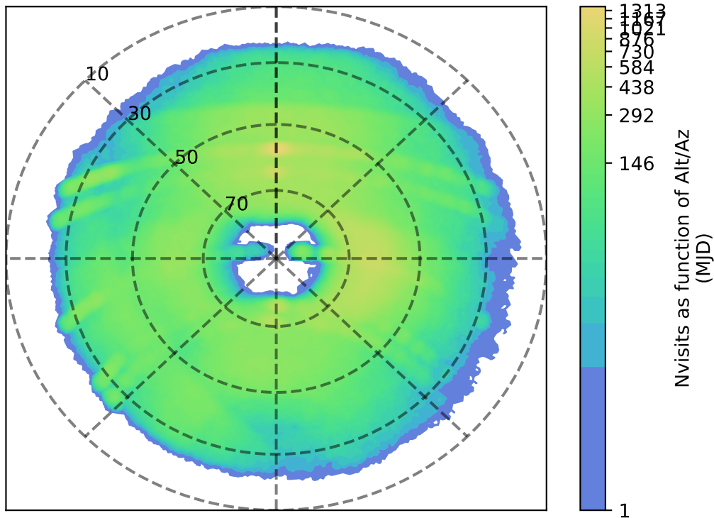
roll_pause_mjdp0_v3.4_10yrs g: Nvisits as function of Alt/Az
