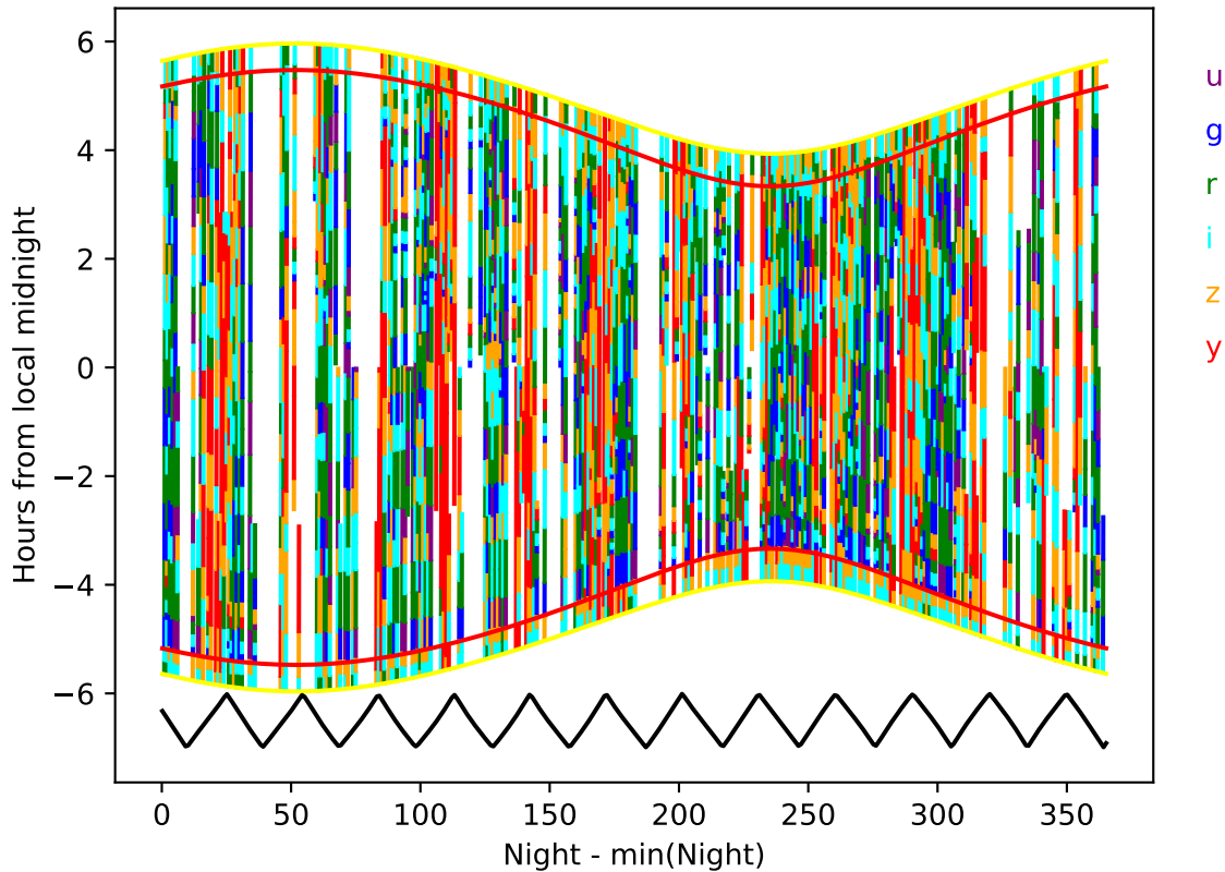
roll_pause_mjdp0_v3.4_10yrs year 7-8: Hourglass
