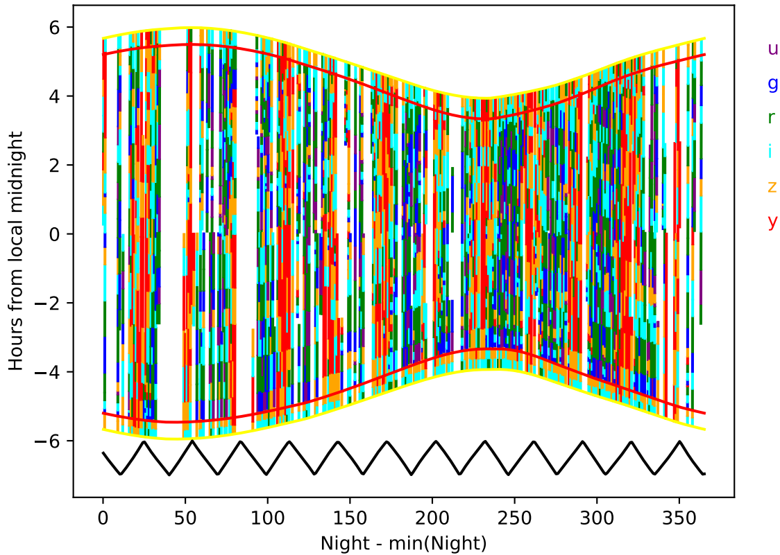
roll_pause_mjdp0_v3.4_10yrs year 4-5: Hourglass
