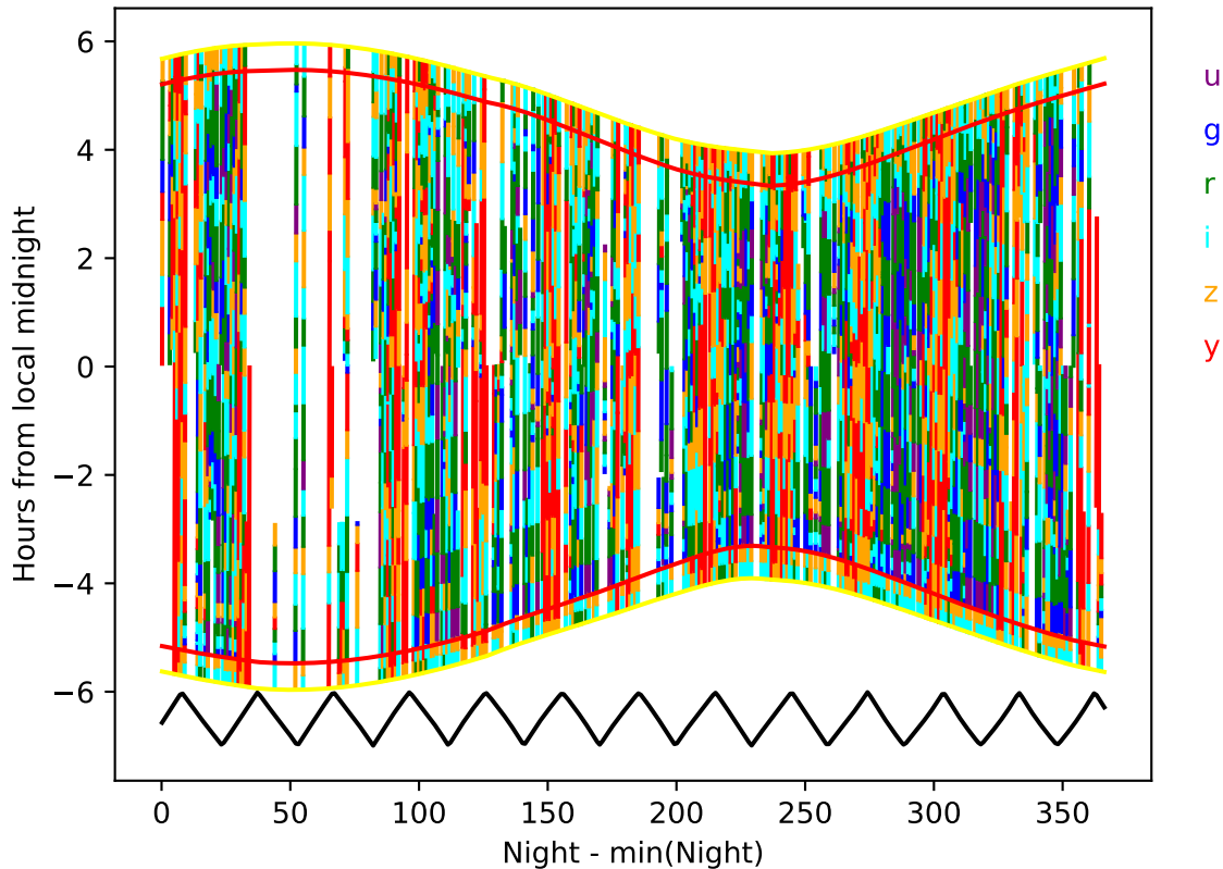
roll_pause_mjdp0_v3.4_10yrs year 3-4: Hourglass
