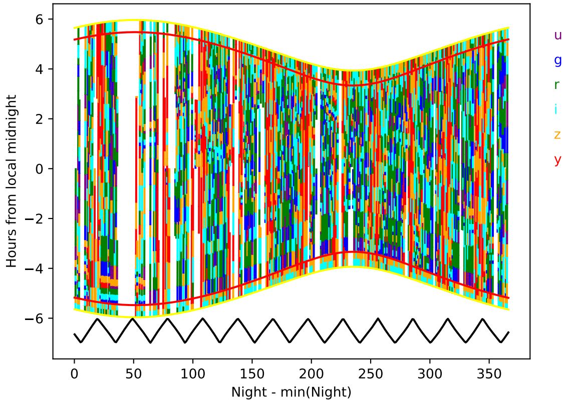
roll_pause_mjdp0_v3.4_10yrs year 2-3: Hourglass
