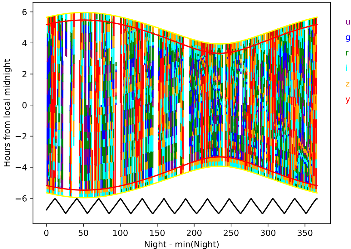
roll_pause_mjdp0_v3.4_10yrs year 0-1: Hourglass
