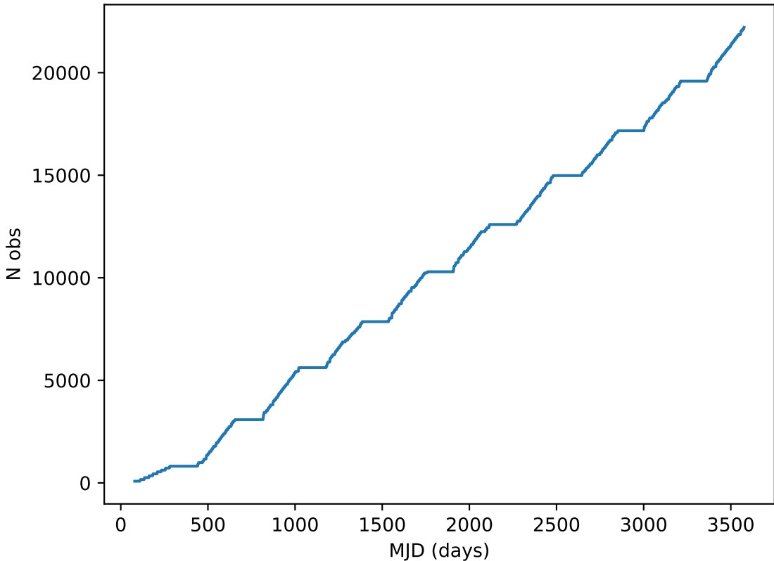
roll_pause_mjdp0_v3.4_10yrs note like DD:XMM_LSS%: Cumulative
