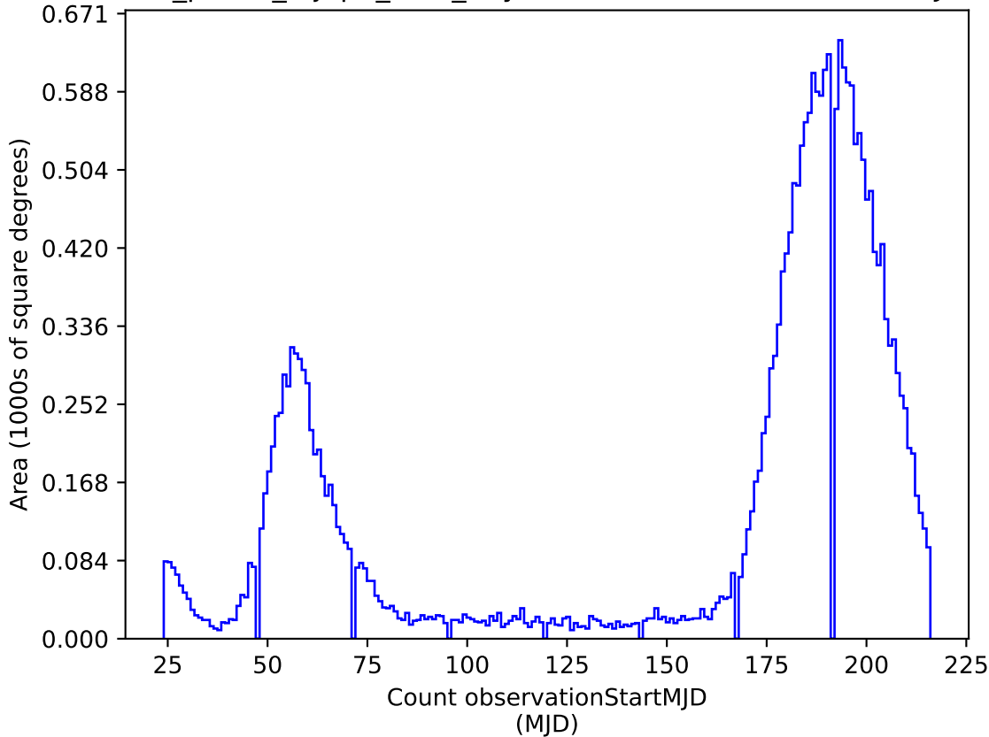
roll_pause_mjdp0_v3.4_10yrs i: Count observationStartMJD
