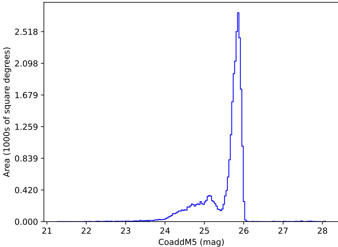
roll_pause_mjdp0_v3.4_10yrs z: CoaddM5
