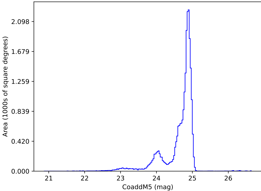
roll_pause_mjdp0_v3.4_10yrs y: CoaddM5
