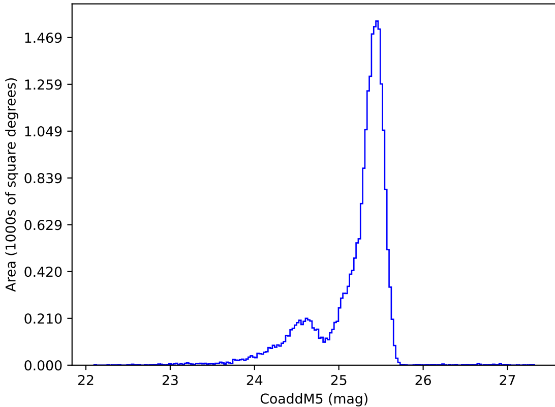
roll_pause_mjdp0_v3.4_10yrs u: CoaddM5
