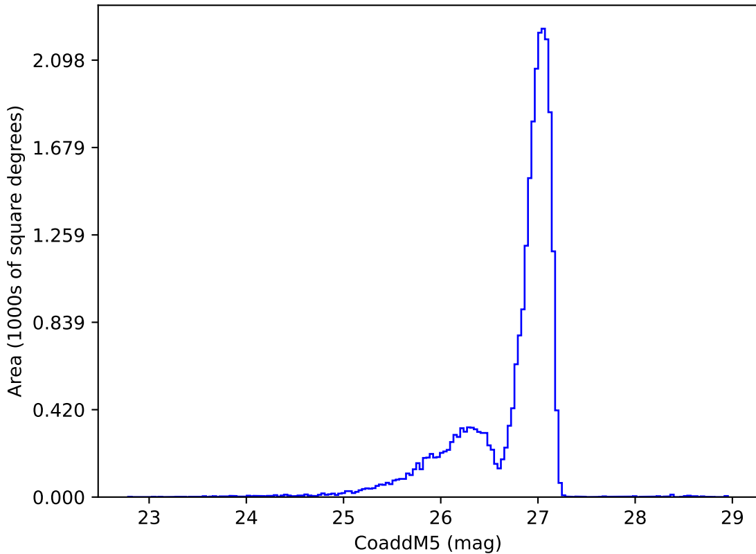
roll_pause_mjdp0_v3.4_10yrs r: CoaddM5
