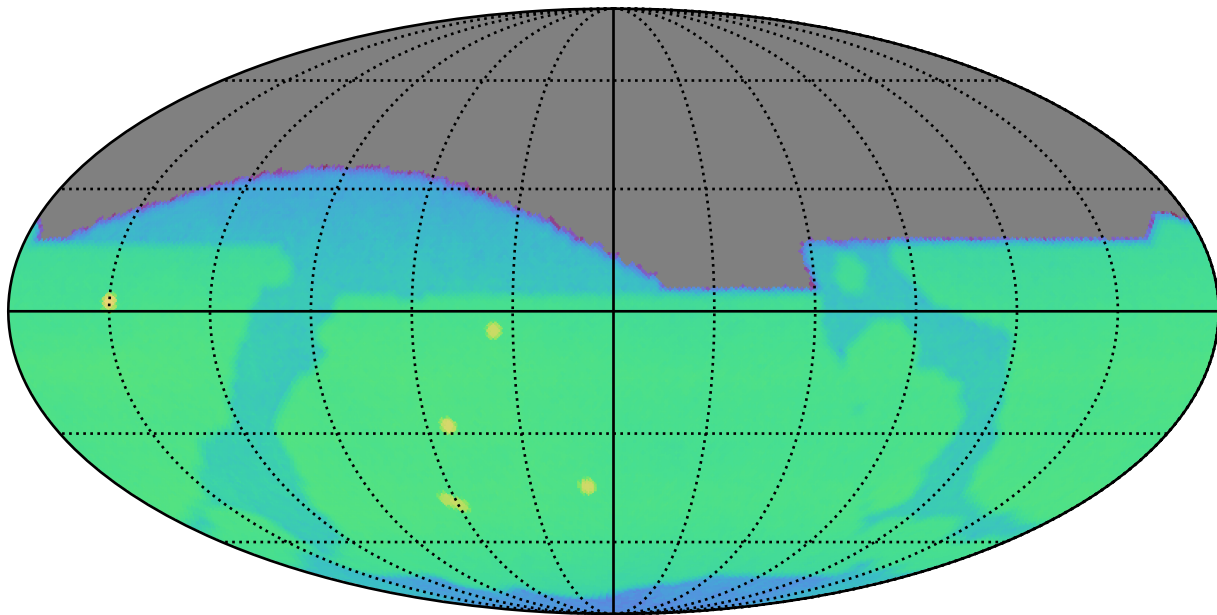
roll_pause_mjdp0_v3.4_10yrs i: CoaddM5
