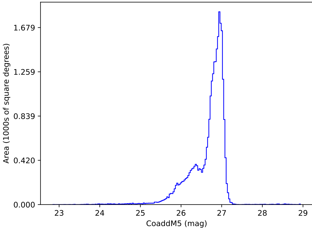
roll_pause_mjdp0_v3.4_10yrs g: CoaddM5
