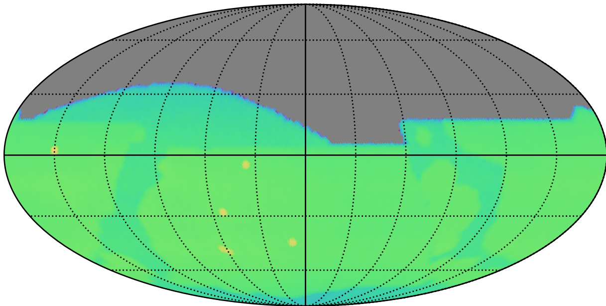
roll_pause_mjdp0_v3.4_10yrs : CoaddM5
