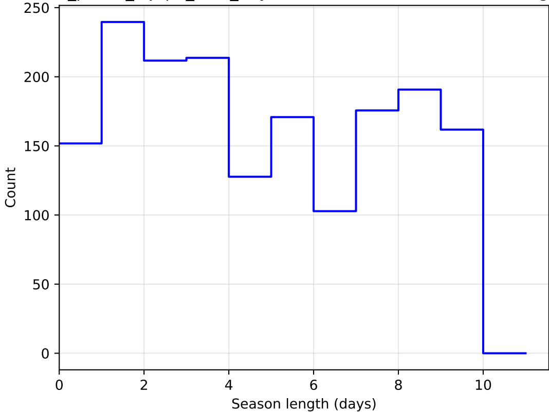
roll_pause_mjdp0_v3.4_10yrs DD:WFD all bands: SeasonLength
