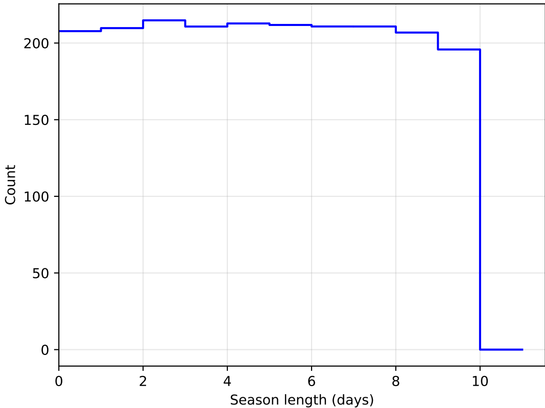
roll_pause_mjdp0_v3.4_10yrs DD:EDFS all bands: SeasonLength
