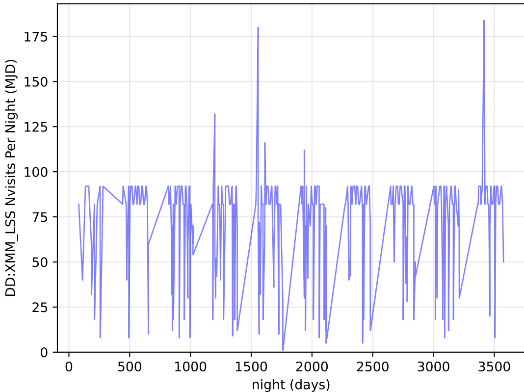
roll_pause_mjdp0_v3.4_10yrs all bands: DD:XMM_LSS Nvisits Per Night
