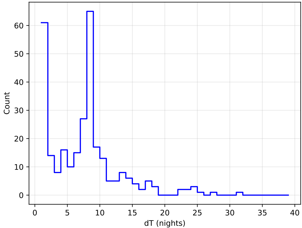
roll_pause_mjdp0_v3.4_10yrs all bands: DD:XMM_LSS Delta Nights Histogram
