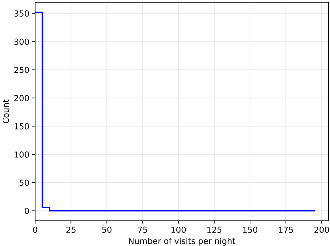
roll_pause_mjdp0_v3.4_10yrs all bands: DD:WFD NVisitsPerNight
